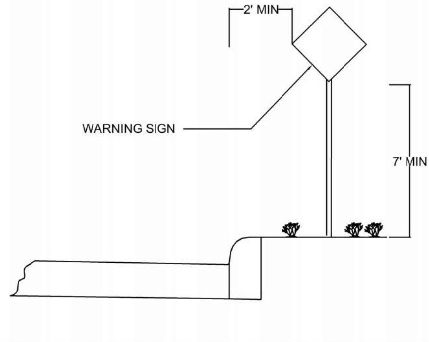
TYPICAL SIGN DETAIL
